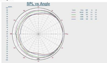
Direction Diagram:
